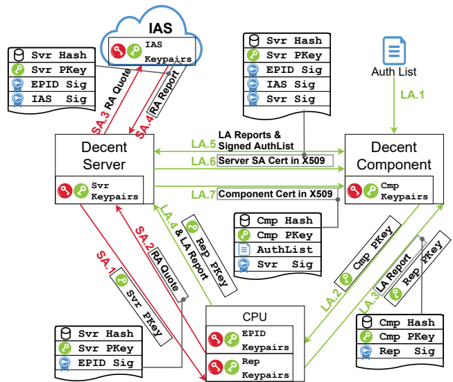
Figure 6: Process of creating certificates for the Decent Component authentication
