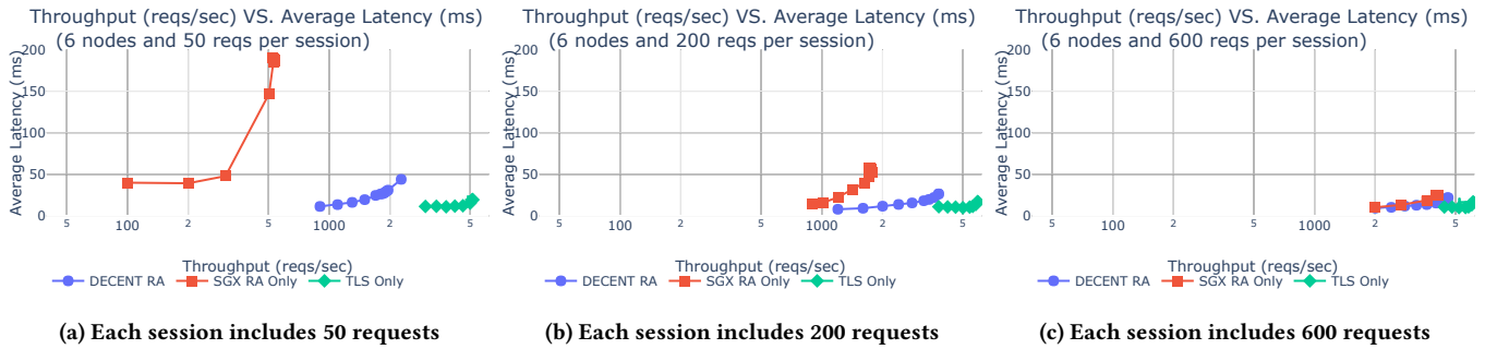
Figure 11: Average latency versus throughput
