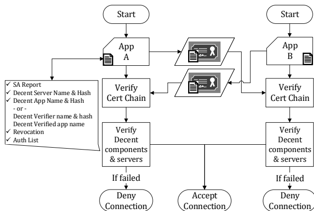
Figure 12: Decent handshake workflow
