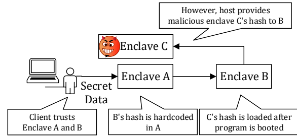
Figure 3: Allowing hosts to authorize enclaves independently could permit flows to malicious enclaves.
