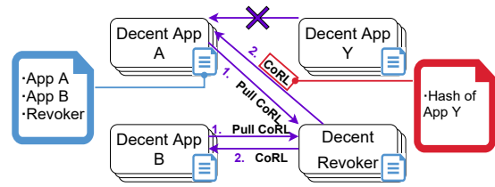
Figure 8: Procedures for the revoker
