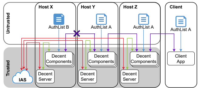
Figure 5: Overview of the Decent Framework; trust model shown is from the perspective of a client
