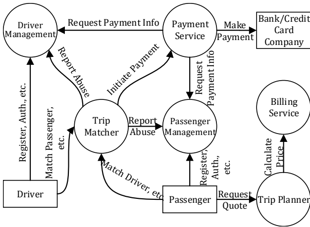
Figure 4: DecentRide, a decentralized ridesharing service.
